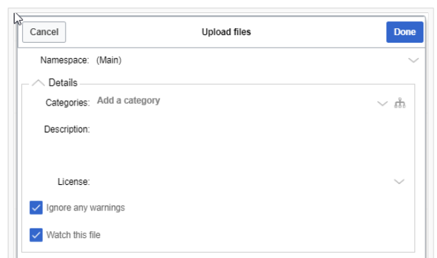
Upload dialog
