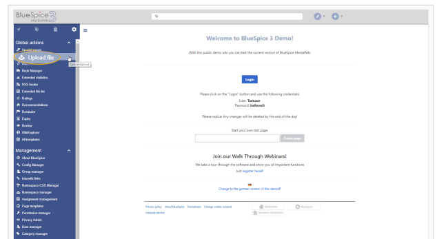
Uploading files
